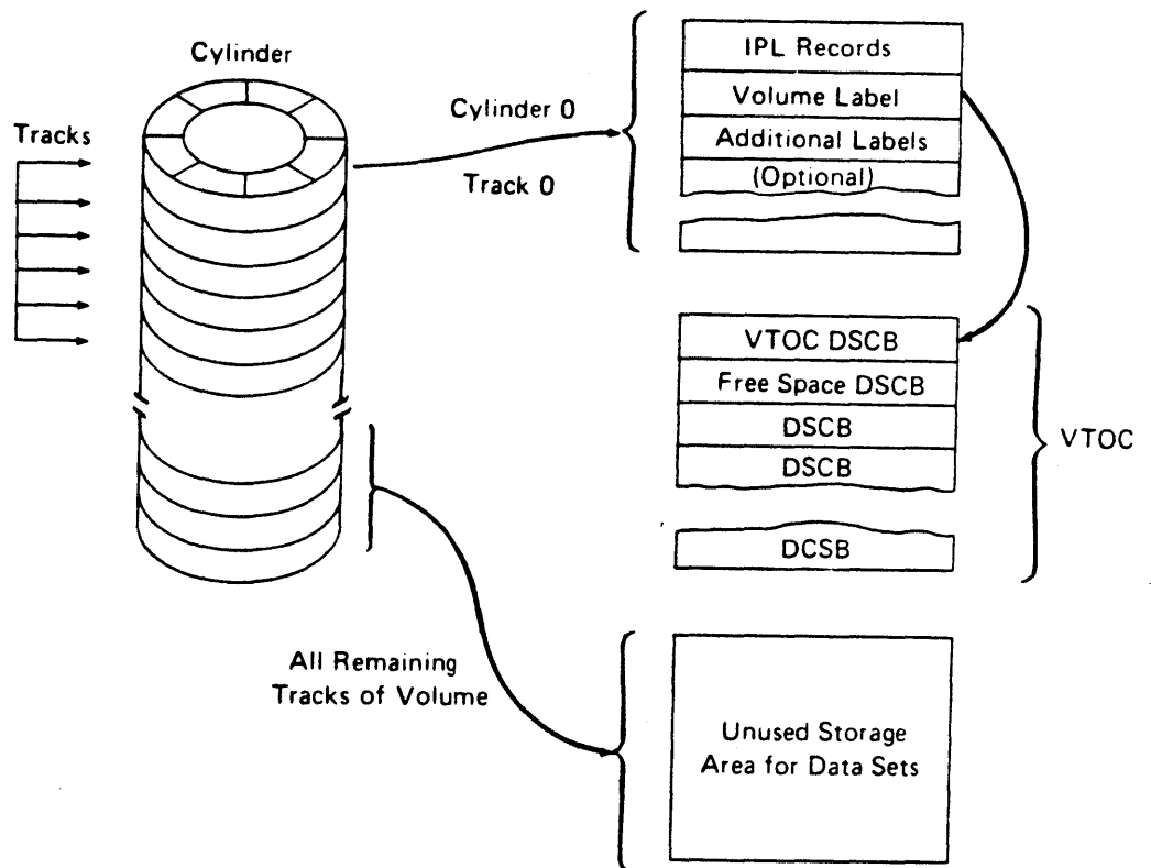
Figure 55. Direct Access Labeling
