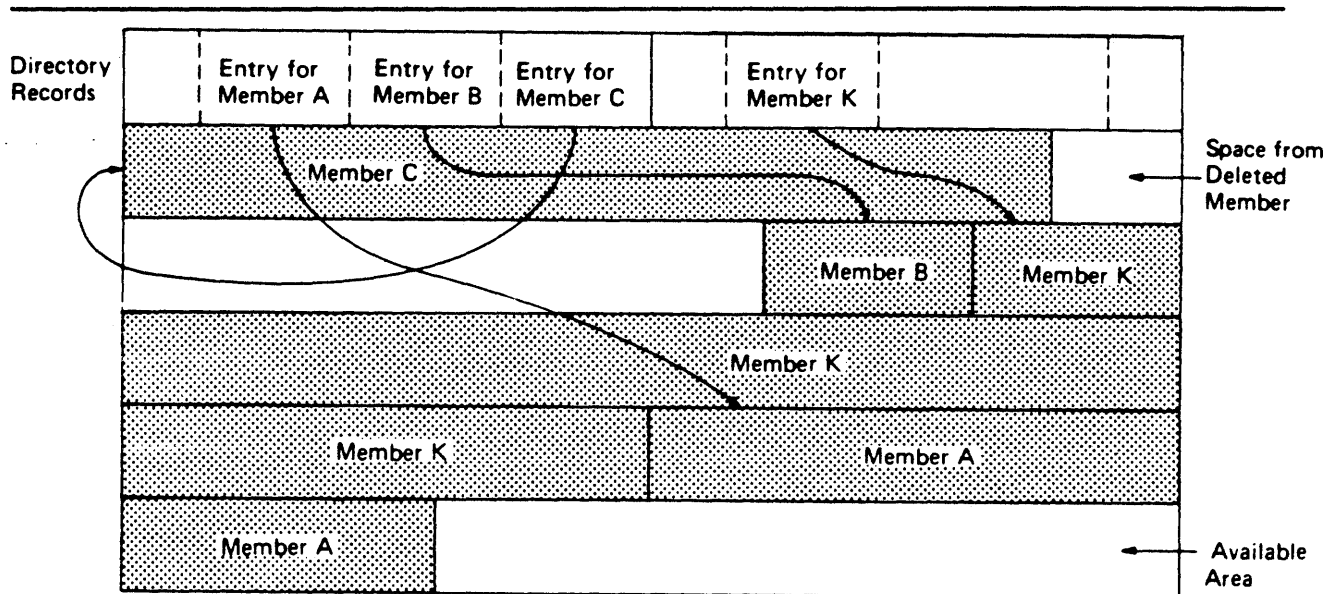
Figure 34. A Partitioned Data Set
