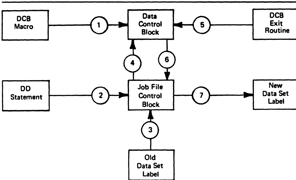
Figure 14. Sources and Sequence of Operations for Completing the Data Control Block
