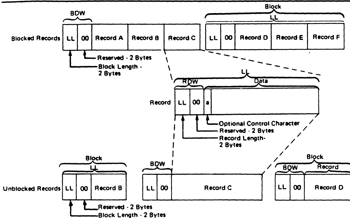
Figure 5. Nonspanned, Format-V Records
