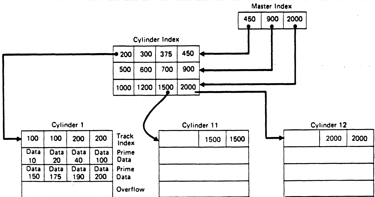
Figure 46. Indexed Sequential Data Set Organization
