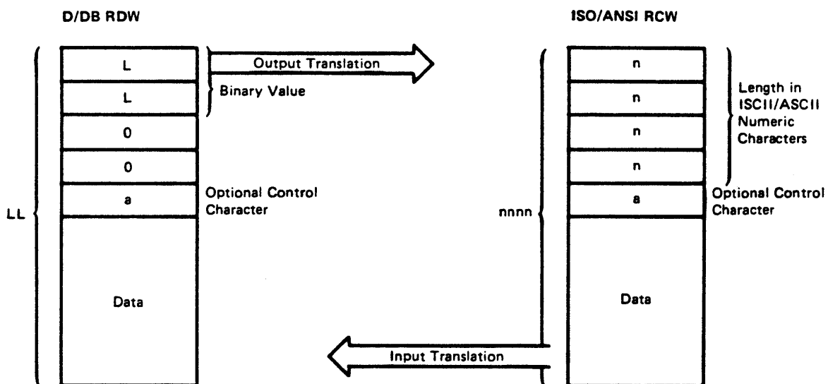
Figure 60. Translation of ISO/ANSI/FIPS Record Control Word to D/DB Record Descriptor Word
