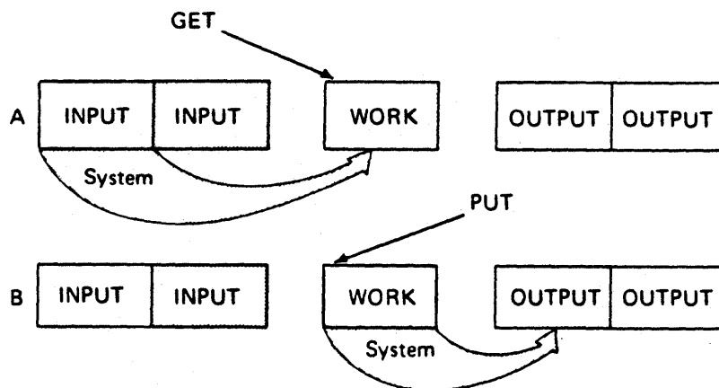
Figure 30. Simple Buffering with MACRF=GM and MACRF=PM
