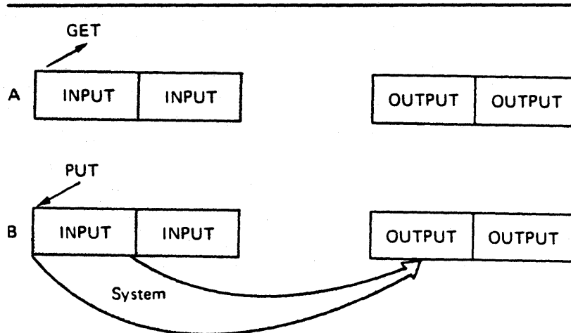
Figure 29. Simple Buffering with MACRF=GL and MACRF=PM
