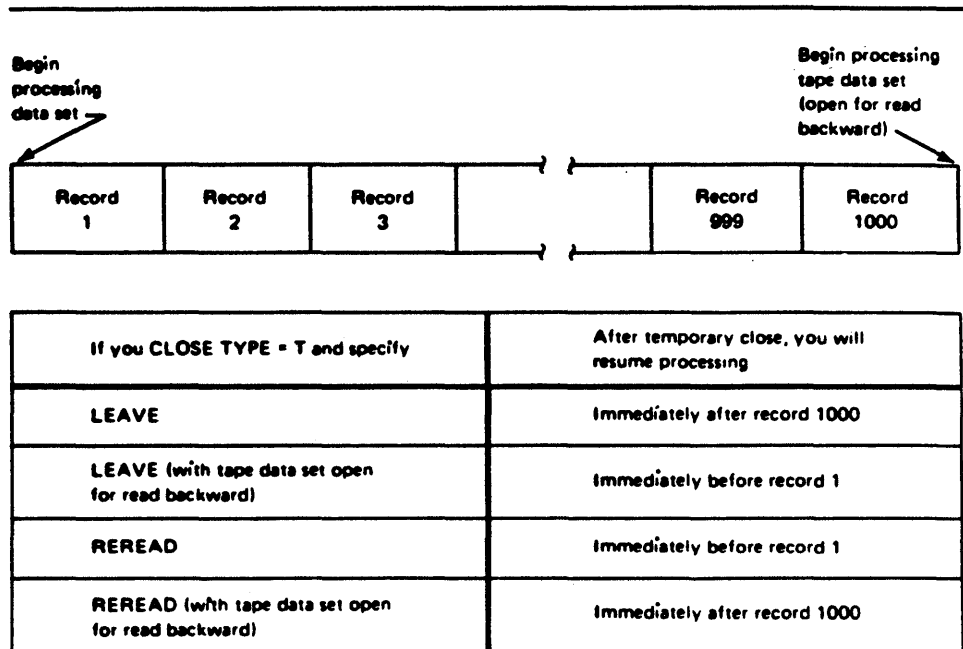
Figure 17. Record Processed When LEAVE or REREAD Is Specified for CLOSE TYPE=T
