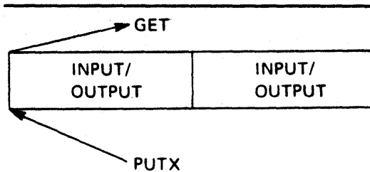
Figure 32. Simple Buffering with MACRF=GL and MACRF=PM-UPDAT Mode
