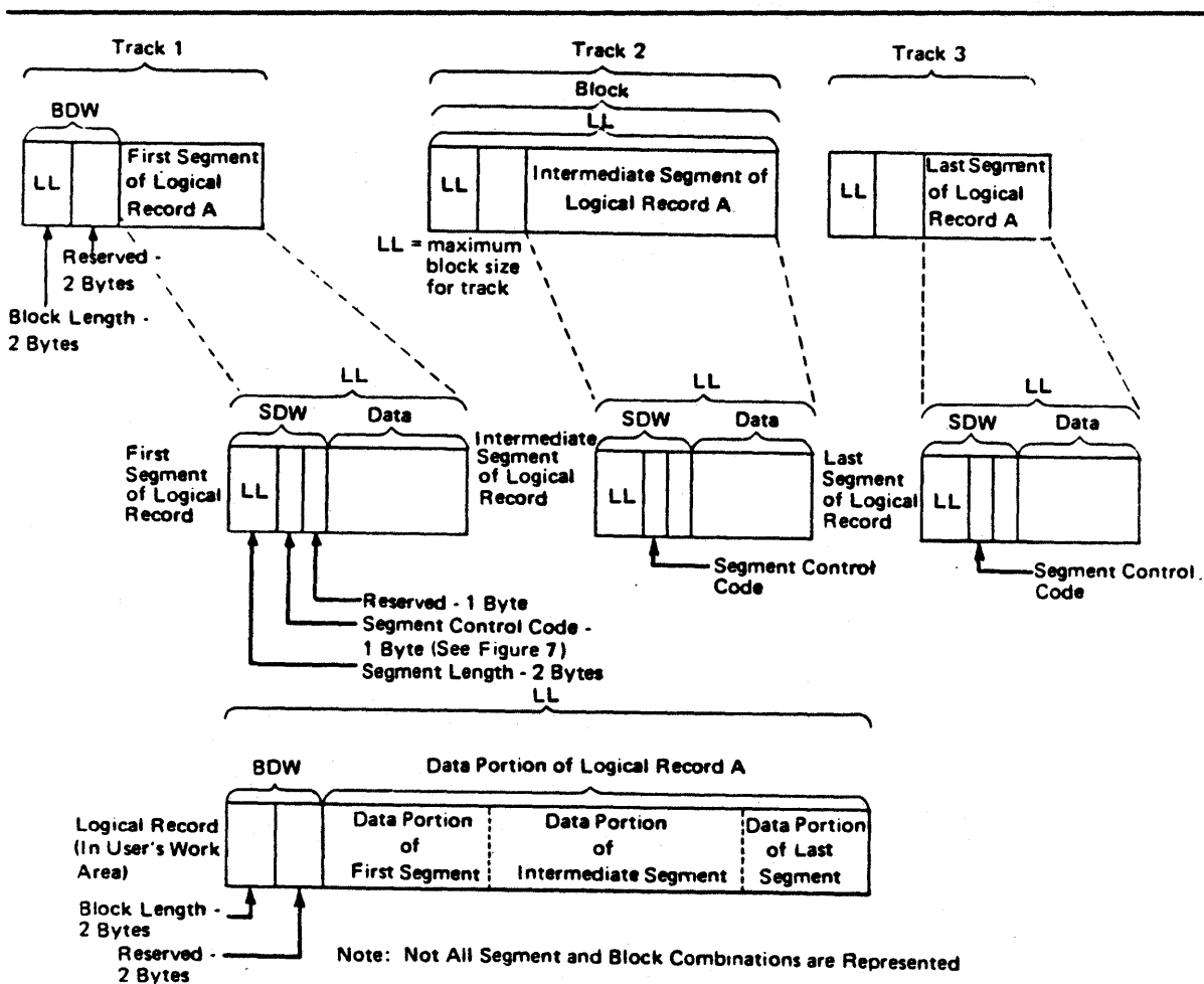
Figure 8. Spanned Format-V Records for BDAM Data Sets
