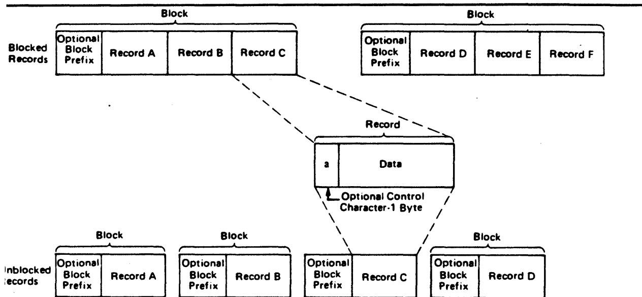
Figure 4. Fixed-Length Records for ISO/ANSI/FIPS Tapes
