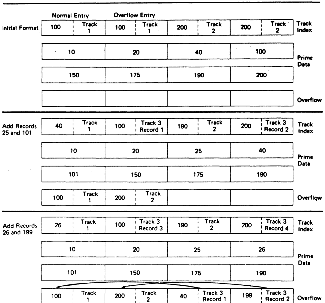
Figure 53. Adding Records to an Indexed Sequential Data Set
