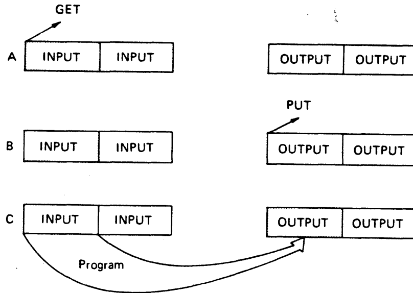
Figure 31. Simple Buffering with MACRF=GL and MACRF=PL
