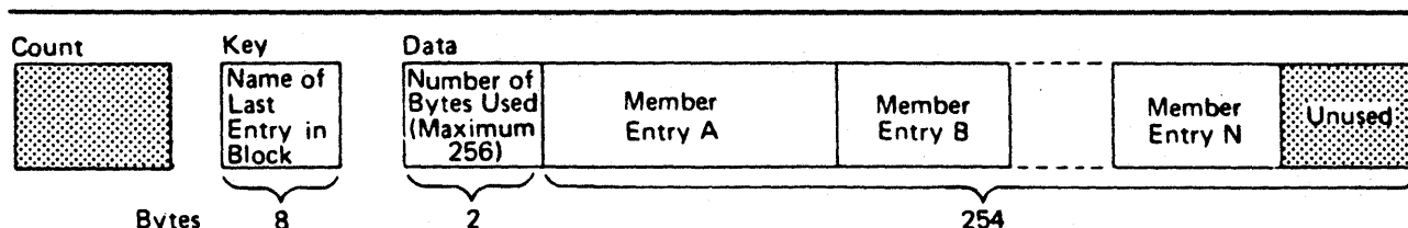
Figure 35. A Partitioned Data Set Directory Block
