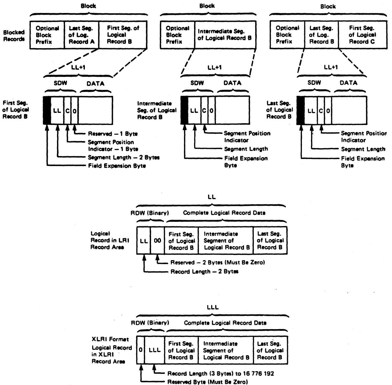
Figure 10. Spanned Variable-Length (Format-DS) Records for ISO/ANSI/FIPS Tapes
