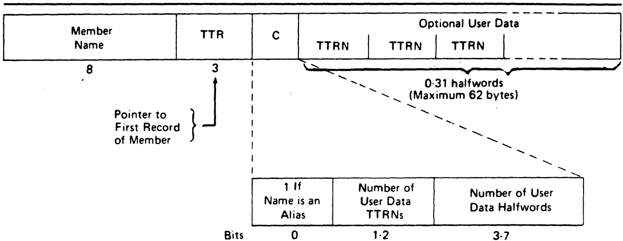
Figure 36. A Partitioned Data Set Directory Entry
