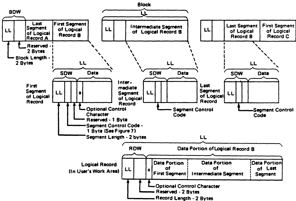
Figure 6. Spanned Format-VS Records (Sequential Access Method)
