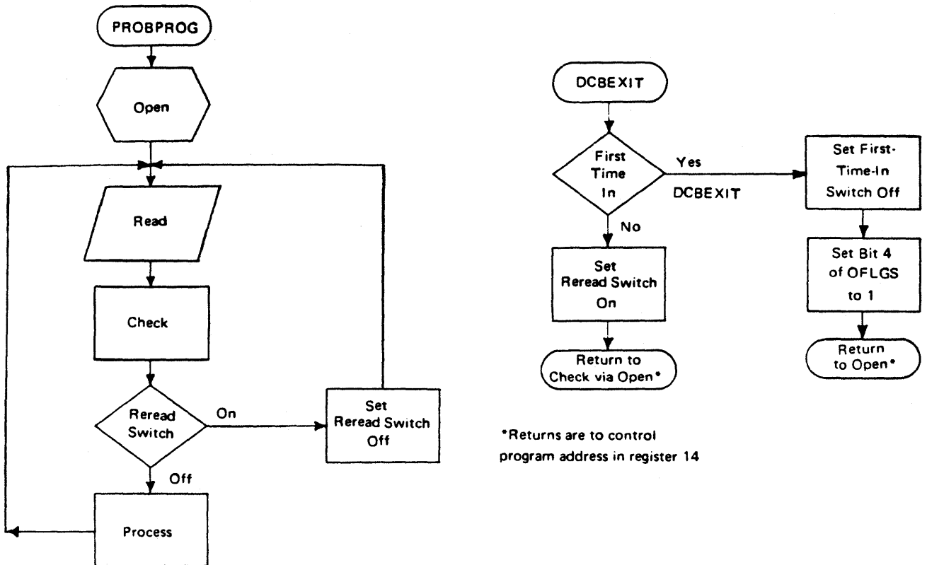
Figure 25. Reissuing a READ or GET for Unlike Concatenated Data Sets
