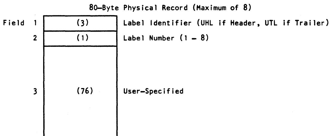
Figure 57. User Header and Trailer Labels
