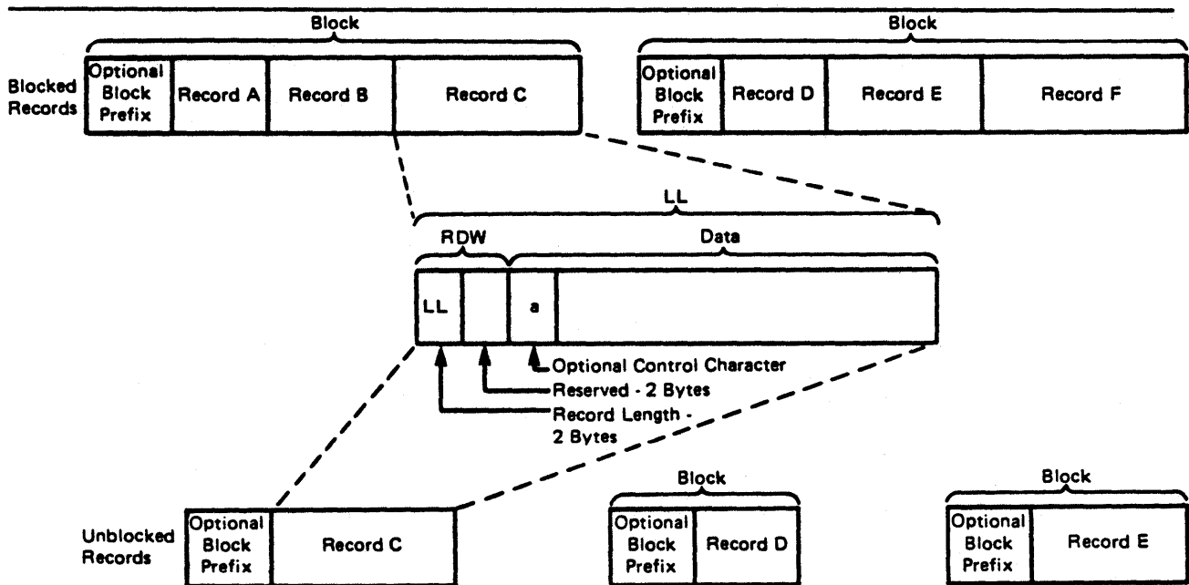
Figure 9. Nonspanned Format-D Records for ISO/ANSI/FIPS Tapes
